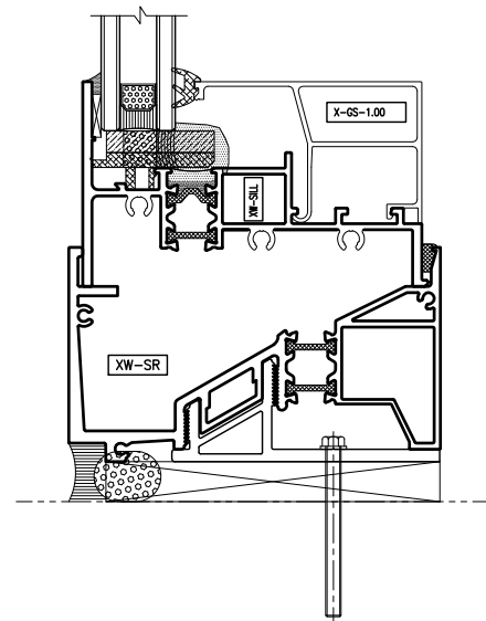
3 Horizontal Detail - Fixed At Sill
