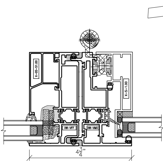
6 Vertical Detail - Fixed / Casement Hinge Side
