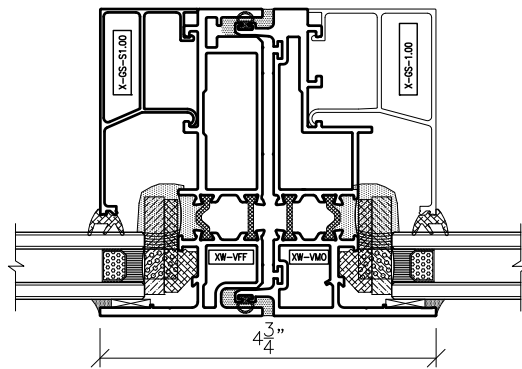
5 Vertical Detail - Fixed / Fixed Below or Above Sash
