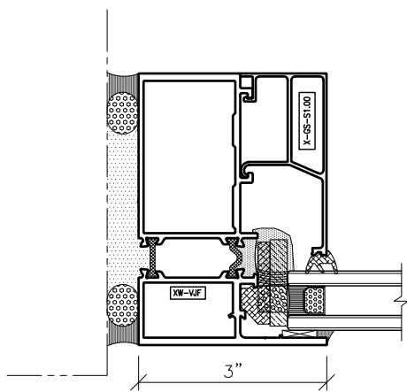
4 Vertical Detail - Jamb
