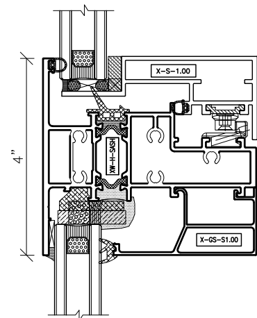
2 Horizontal Detail - Casement Over Fixed
