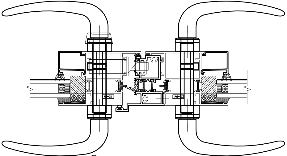
4 Vertical Detail – Inswing Door Handle Side
