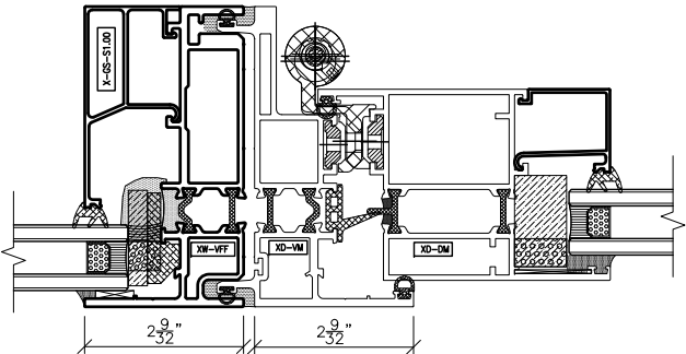
3 Vertical Detail – Inswing Door Hinge Side
