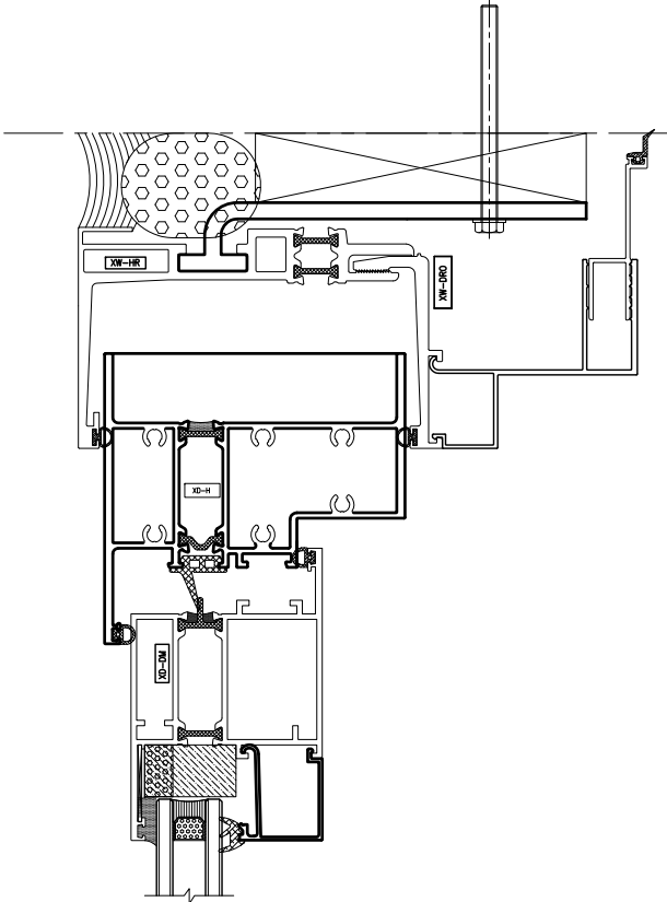
1 Horizontal Detail – Inswing Door At Head
