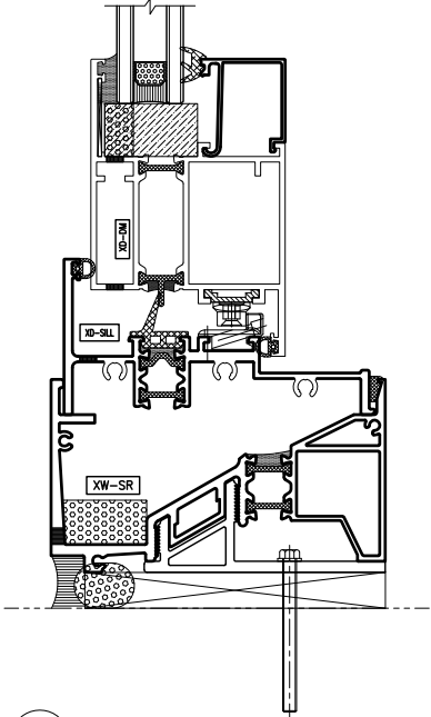
2 Horizontal Detail – Inswing Door At Sill
