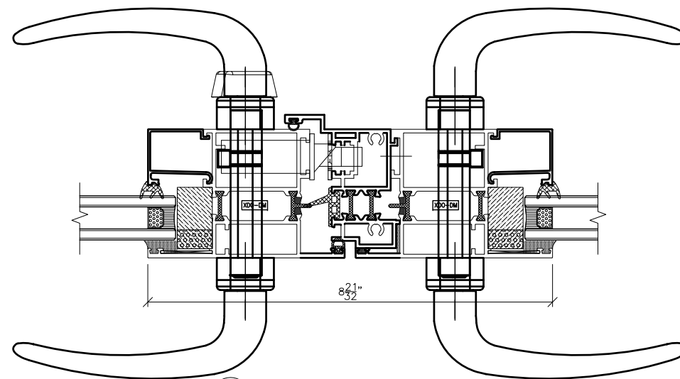
4 Vertical Detail - Outswing Door Handle Side
