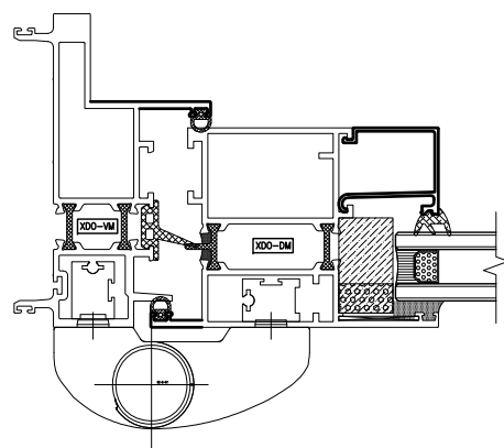
3 Vertical Detail - Outswing Door Hinge Side
