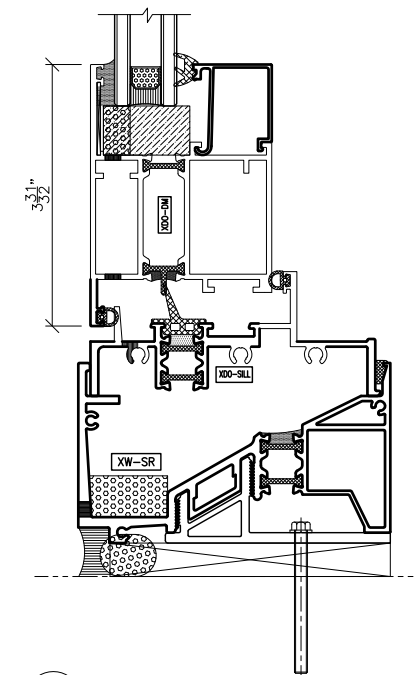
2 Horizontal Detail - Outswing Door At Sill
