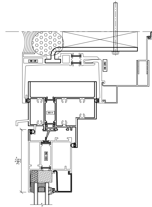
1 Horizontal Detail - Outswing Door At Head
