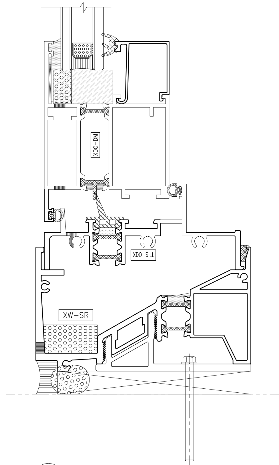
② Standard Profile - Outswing
