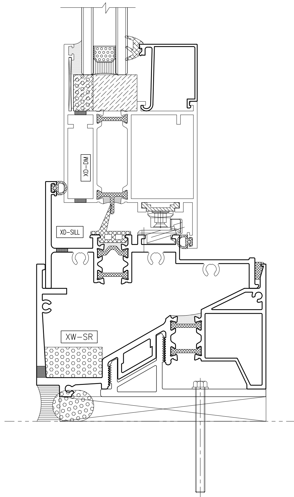
① Standard Profile - Inswing
