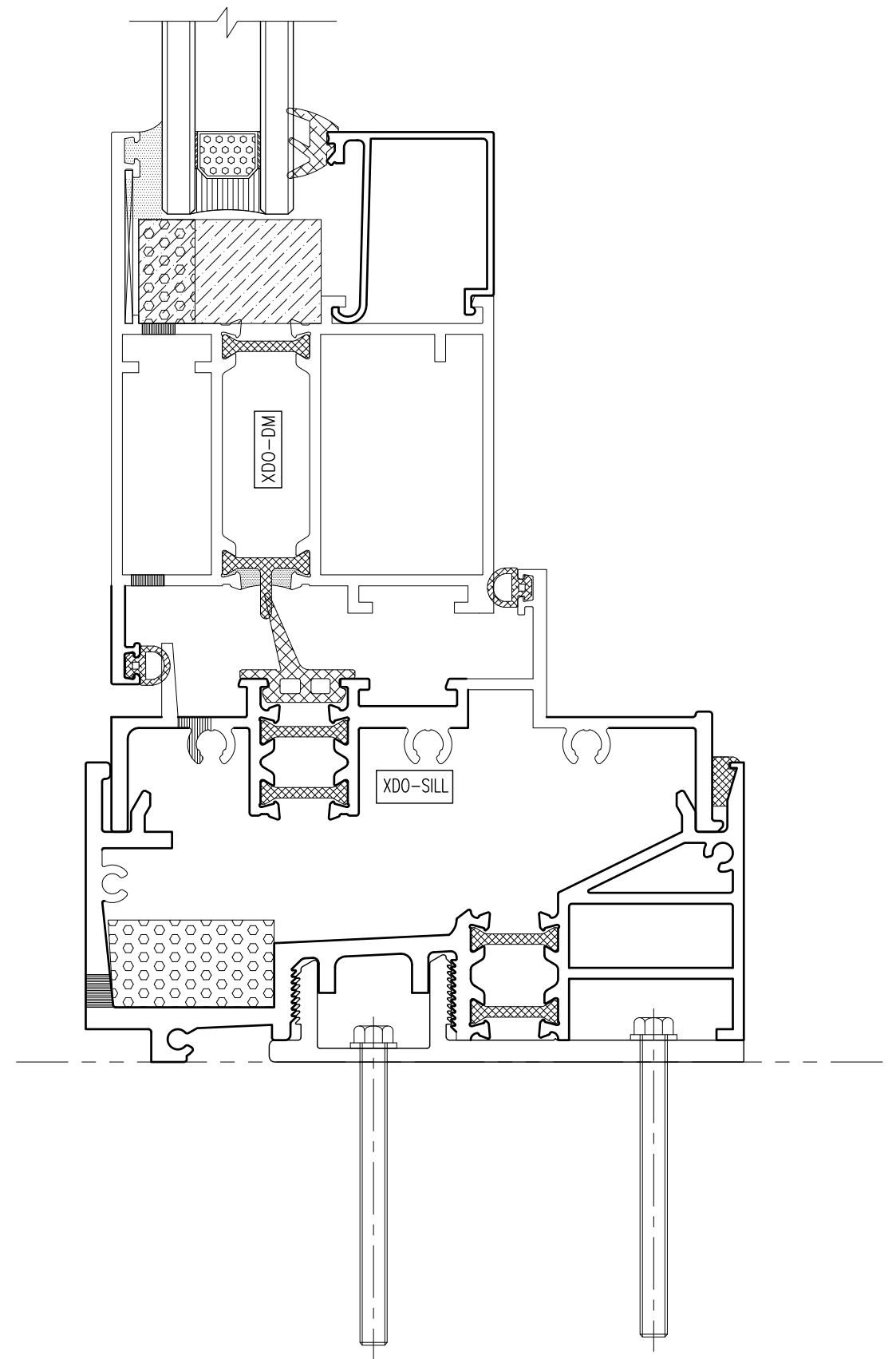
② Low Profile – Outswing
