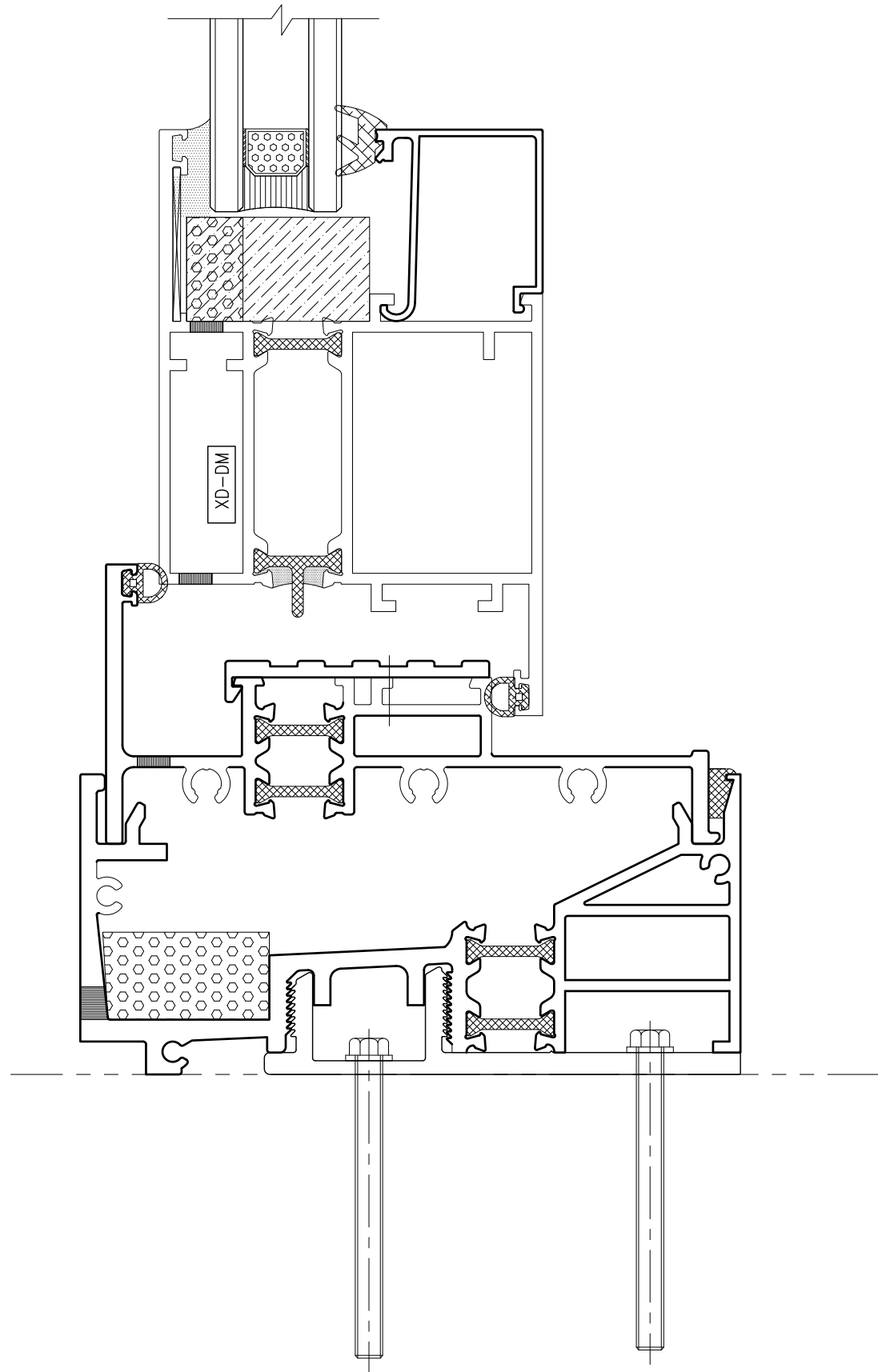
① Low Profile – Inswing
