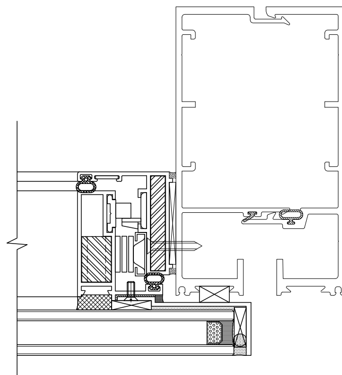
4 Project-Out Detail @ Arm Hinge
