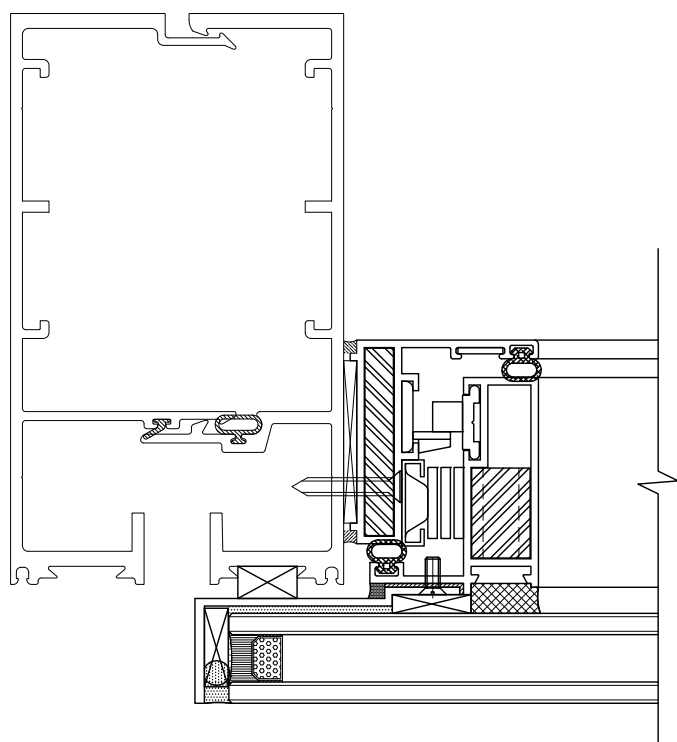
3 Project-Out Detail @ Arm Hinge
