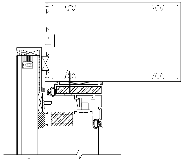
1 Project-Out Detail @ Top Rail
