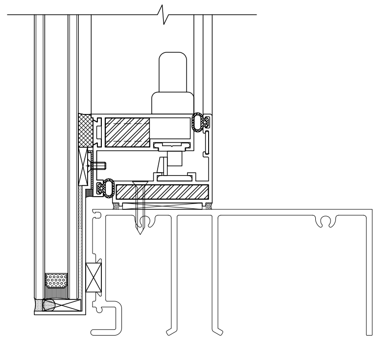
2 Project-Out Detail @ Bottom Rail / Handle
