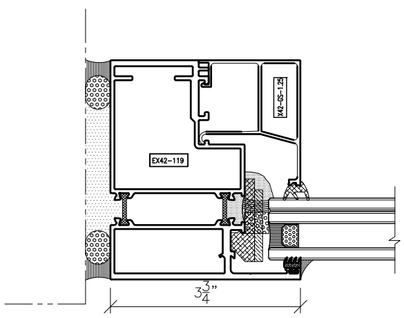
4 Vertical Detail - Jamb
