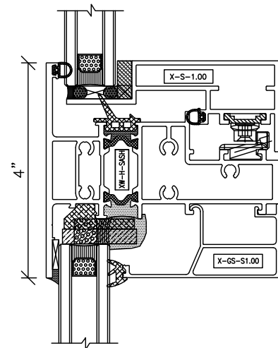
2 Horizontal Detail - Casement Over Fixed
