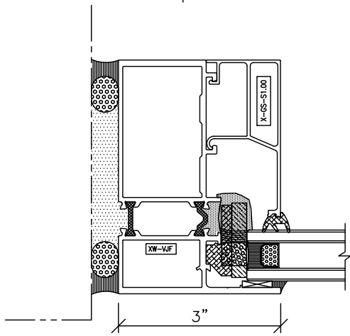
4 Vertical Detail - Jamb
