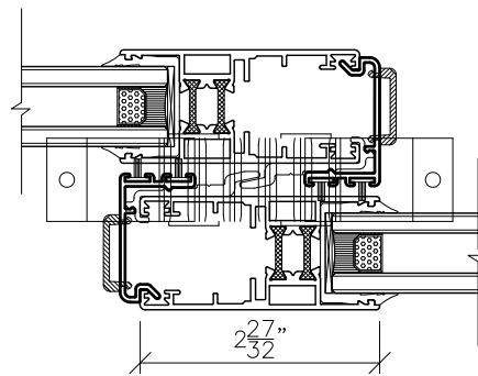
4 Vertical Detail - Intermediate
