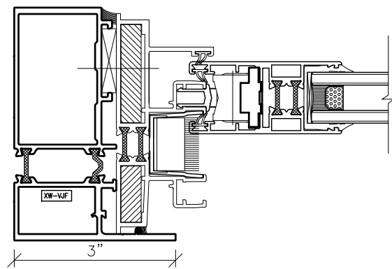
3 Vertical Detail - Jamb
