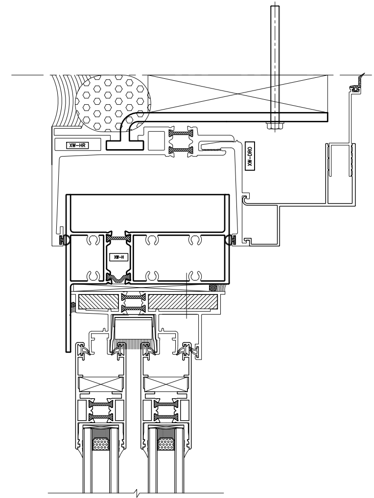
1 Horizontal Detail - Slide At Head
