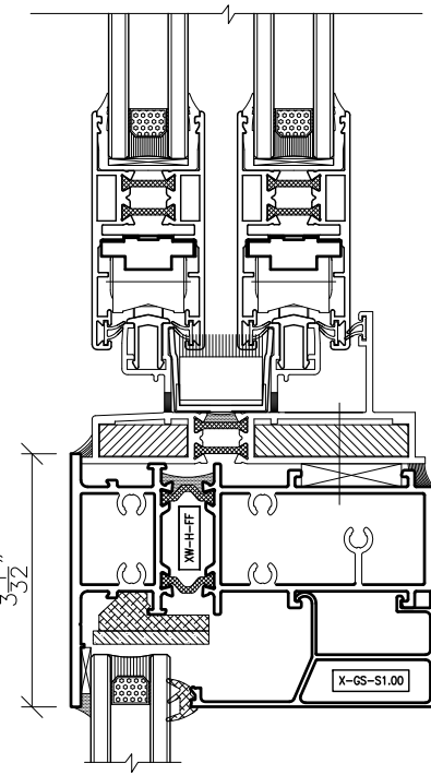
2 Horizontal Detail - Slide At Sill
