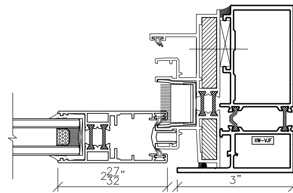
5 Vertical Detail - Jamb
