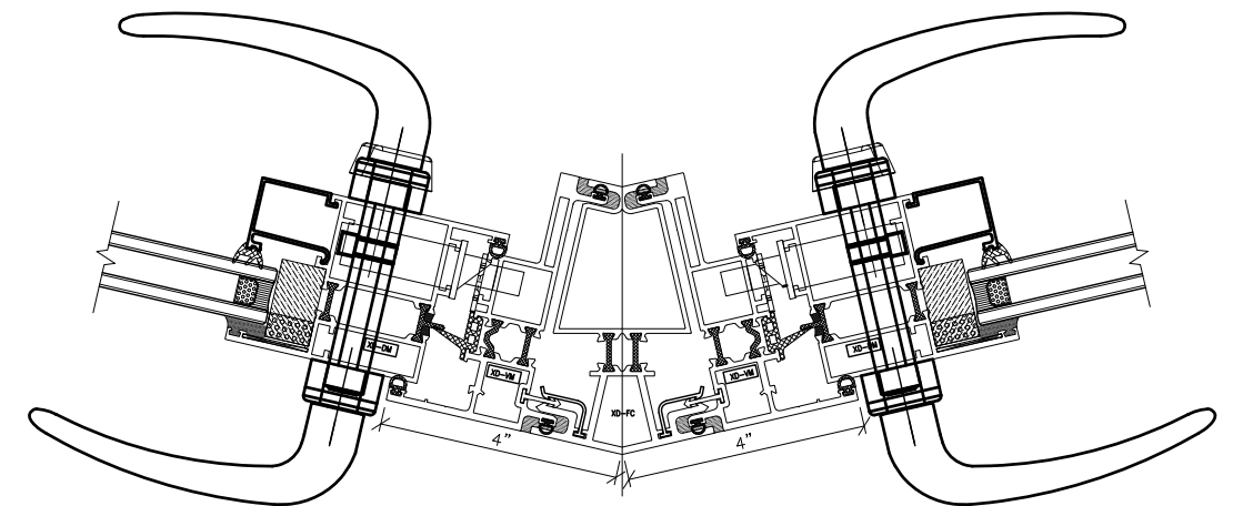
7 FIXED POST BETWEEN DOORS
