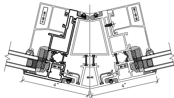
5 FIXED GLASS @ TRANSOM / FIXED GLASS
