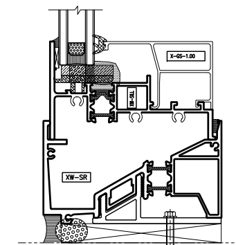
3 Horizontal Detail - Fixed At Sill
