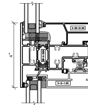
2 Horizontal Detail - Fixed Over Casement
