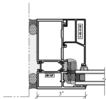
4 Vertical Detail - Jamb
