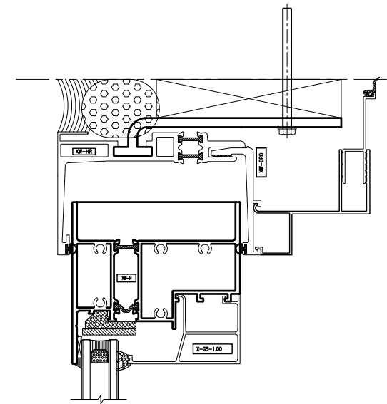
1 Horizontal Detail - Fixed At Ceiling
