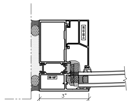
4 Vertical Detail - Jamb
