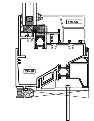
3 Horizontal Detail - Fixed At Sill
