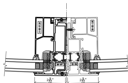
5 FIXED GLASS @ TRANSOM / FIXED GLASS
