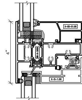
2 Horizontal Detail - Fixed Over Casement
