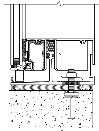
3 Sill Starter
