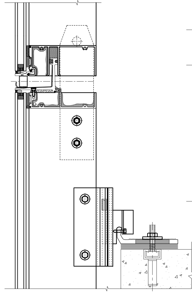
3 Anchor Detail
