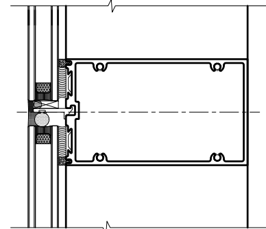
2 Intermediate Horizontal
