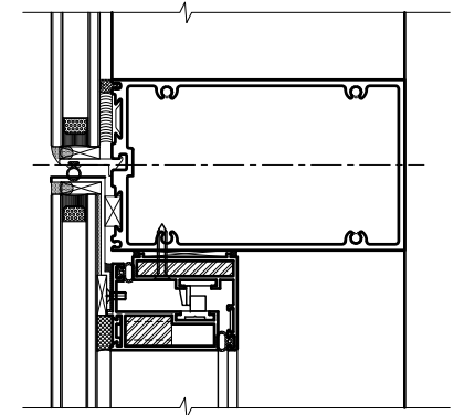
5 PROJECT OUT - Horizontal DETAIL
