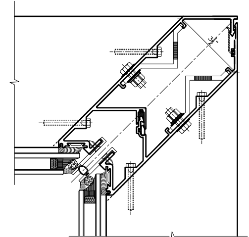
11 Inside Corner
