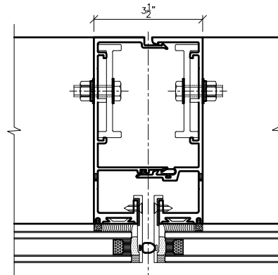
9 Vertical Mullion
