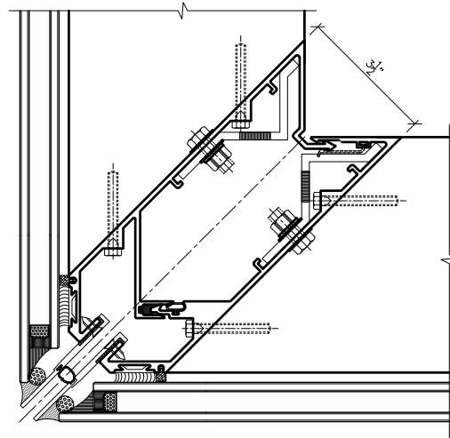
8 Outside Corner
