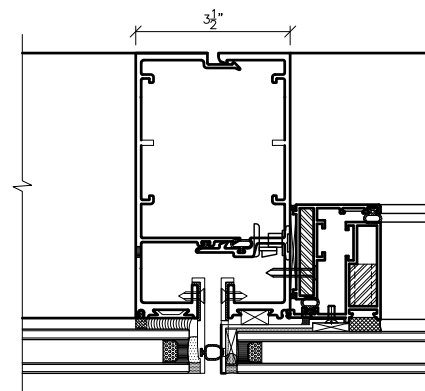
10 PROJECT OUT - VERTICAL DETAIL
