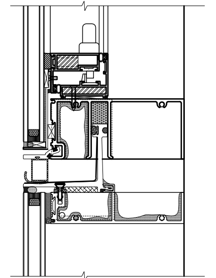
6 PROJECT OUT - Horizontal DETAIL
