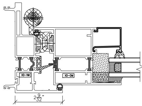
3 Vertical Detail – Inswing Door Hinge Side
