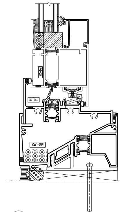
2 Horizontal Detail – Inswing Door At Sill
