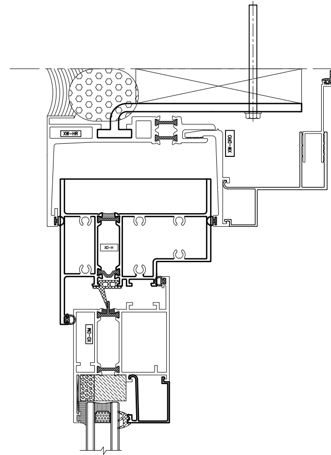
1 Horizontal Detail – Inswing Door At Head
