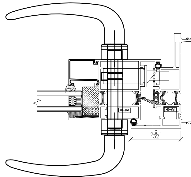
4 Vertical Detail – Inswing Door Handle Side
