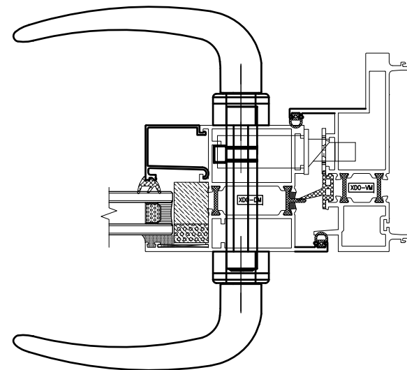
4 Vertical Detail – Outswing Door Handle Side
