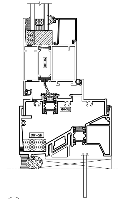
2 Horizontal Detail – Outswing Door At Sill
